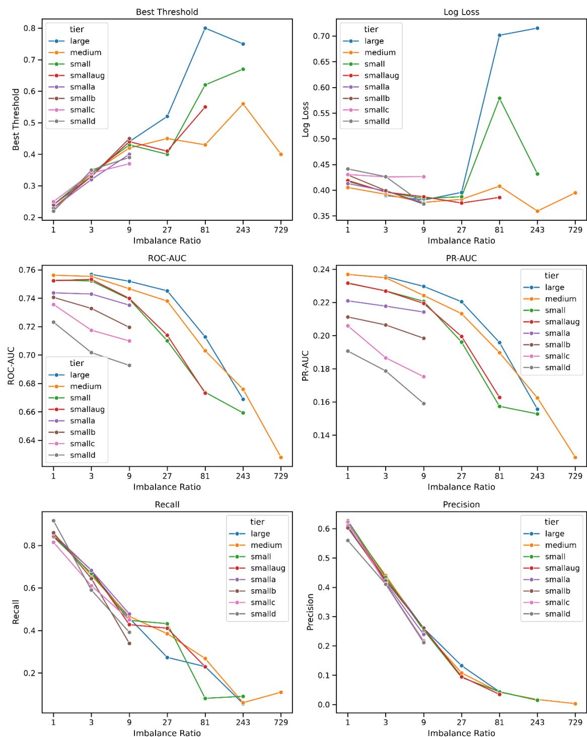
Figure 11. Best threshold, recall and precision vary approximately linearly with \log(\text{IR}) . ROC-AUC and PR-AUC appear to have a more linear correlation to IR. While log-loss is unaffected until IR 81 then become unstable.
