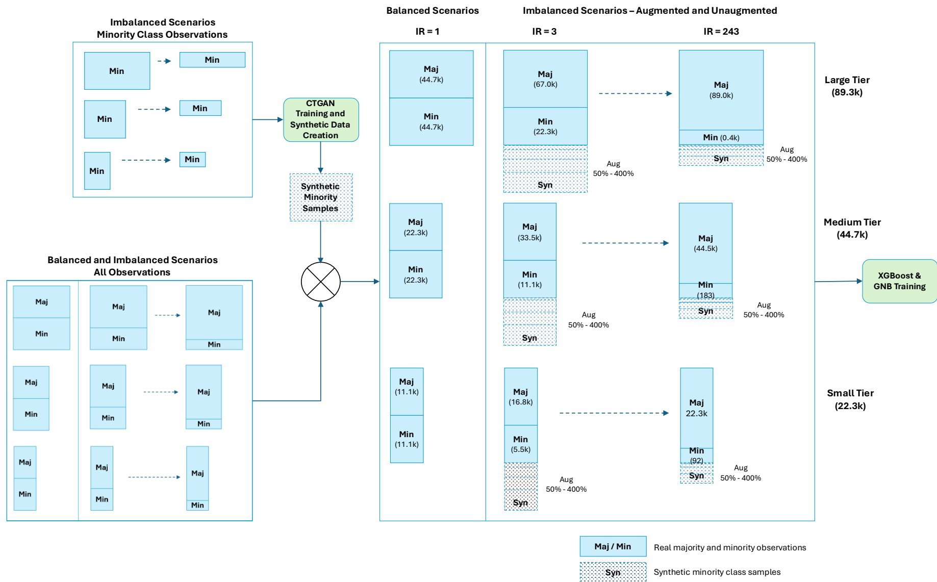
Figure 2. CTGAN is trained using minority samples from imbalanced scenarios, then used to create different levels of synthetic data to augment them.
