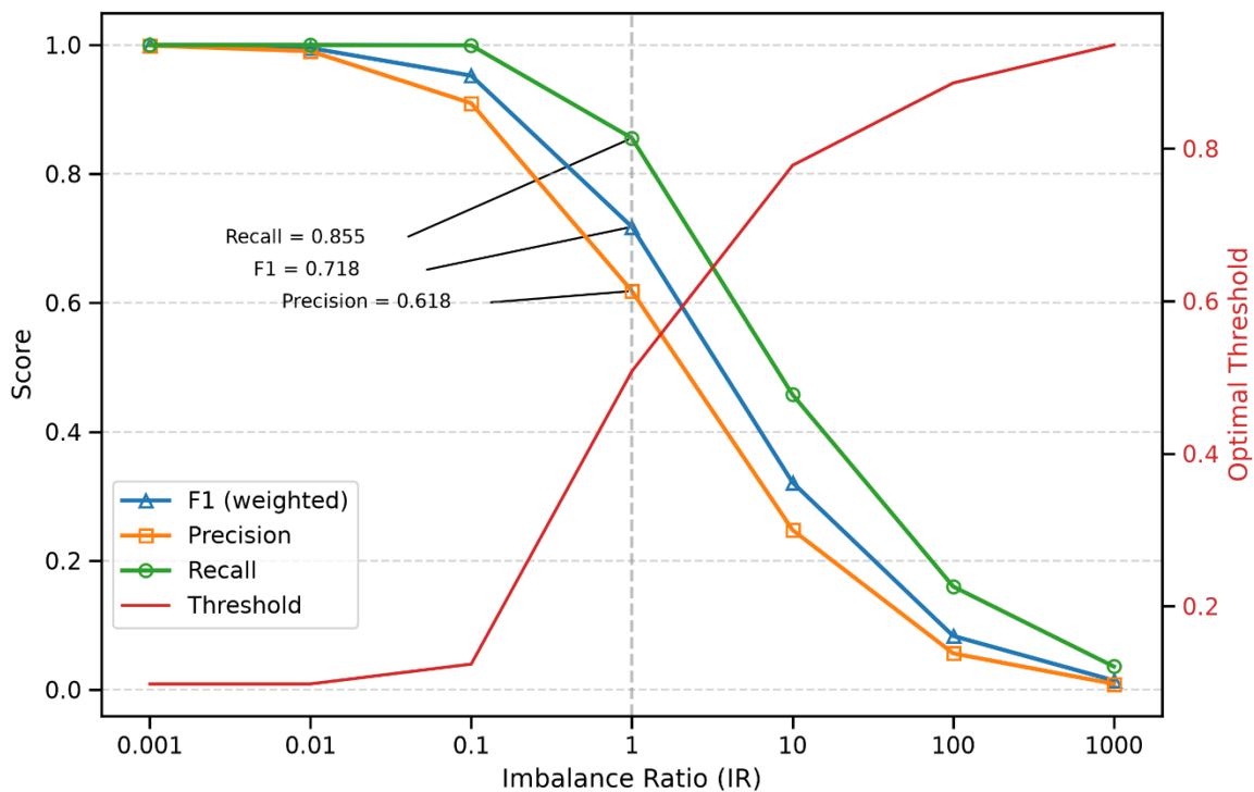
Figure 7. A model trained on a balanced dataset performs well when evaluated in worlds with abundant positive samples ( \text{IR} < 1 ), but its performance deteriorates as the evaluation world becomes increasingly dominated by negative samples. Balancing the training set does not prevent performance collapse under extreme evaluation imbalance.
